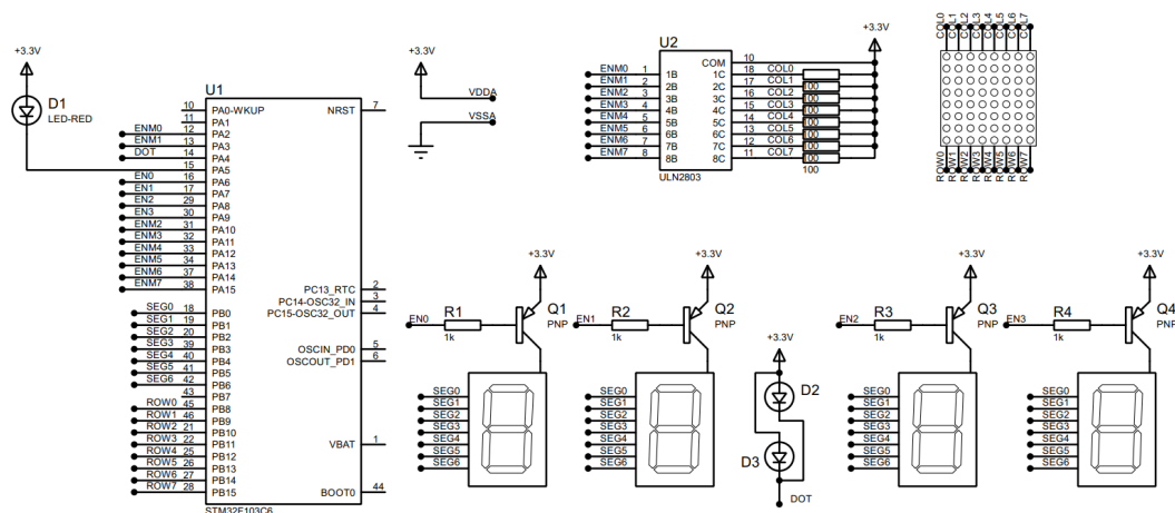
Hình 9: LED matrix is added to the simulation
